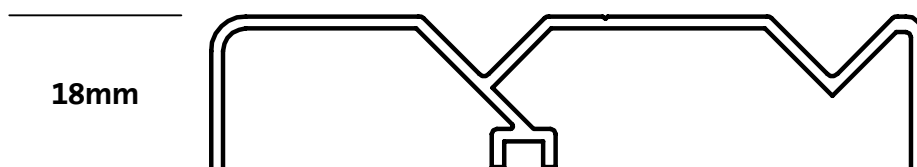
G10 - Silicone Sill
