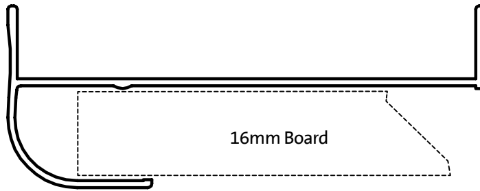
G13 - Curved Jamb
