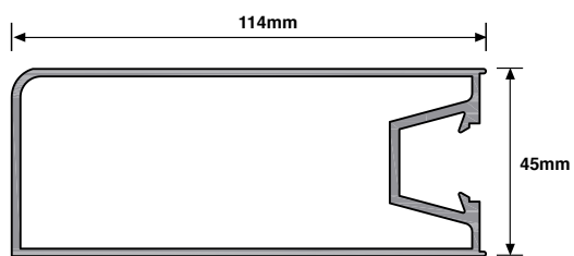
CD-154 - Wide Hinge Stile
