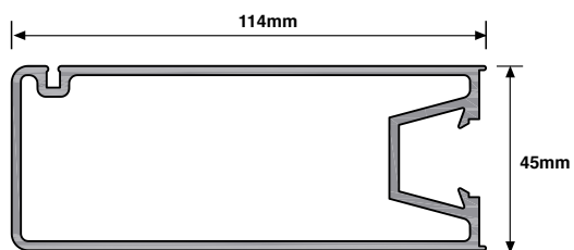
CD-159 - Wide Sliding Stile
