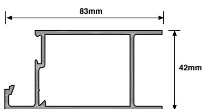
CD-313 - Top Rail
