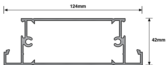
CD-124 - Mid Rail
