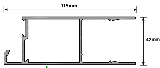
CD-315 - Bottom/Top Rail
