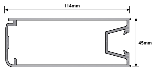
CD-155 - Wide Lock Stile
