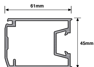
CD-312 - Narrow Lock Stile
