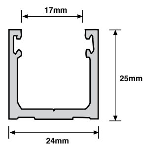
503 - Glazing Channel
