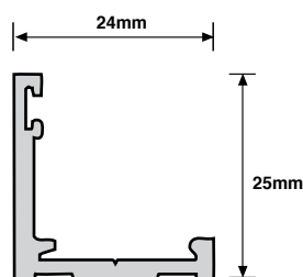
501 - Glazing Adapter
