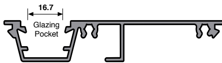
SIG 2009 - Glazing Adaptor
